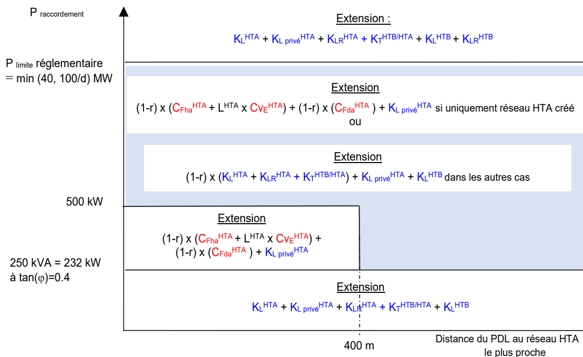
Figure 3 Composantes de la facturation des extensions HTA
